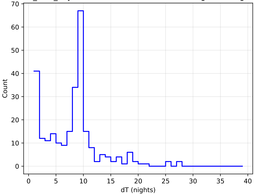
octo_v3.4_10yrs all bands: DD:ELAISS1 Delta Nights Histogram
