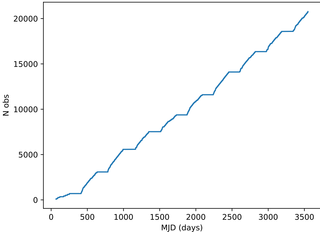
octo_v3.4_10yrs all bands: DD:ELAISS1 Cumulative NVisits
