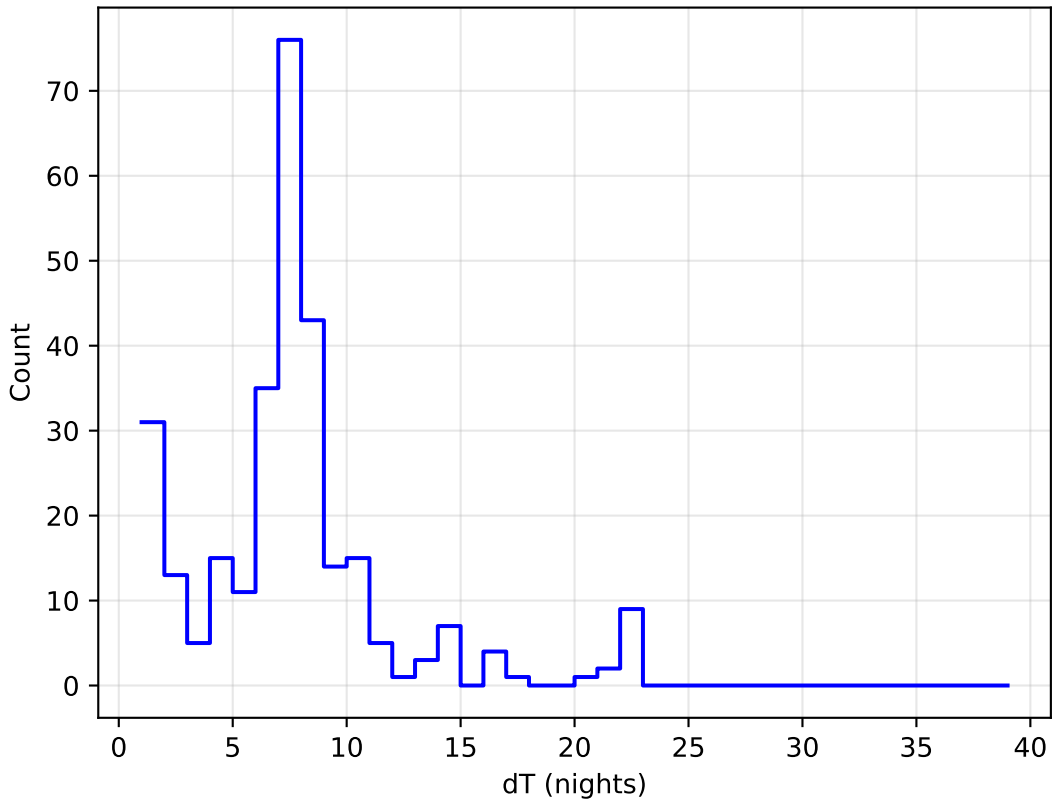
octo_v3.4_10yrs all bands: DD:EDFS Delta Nights Histogram
