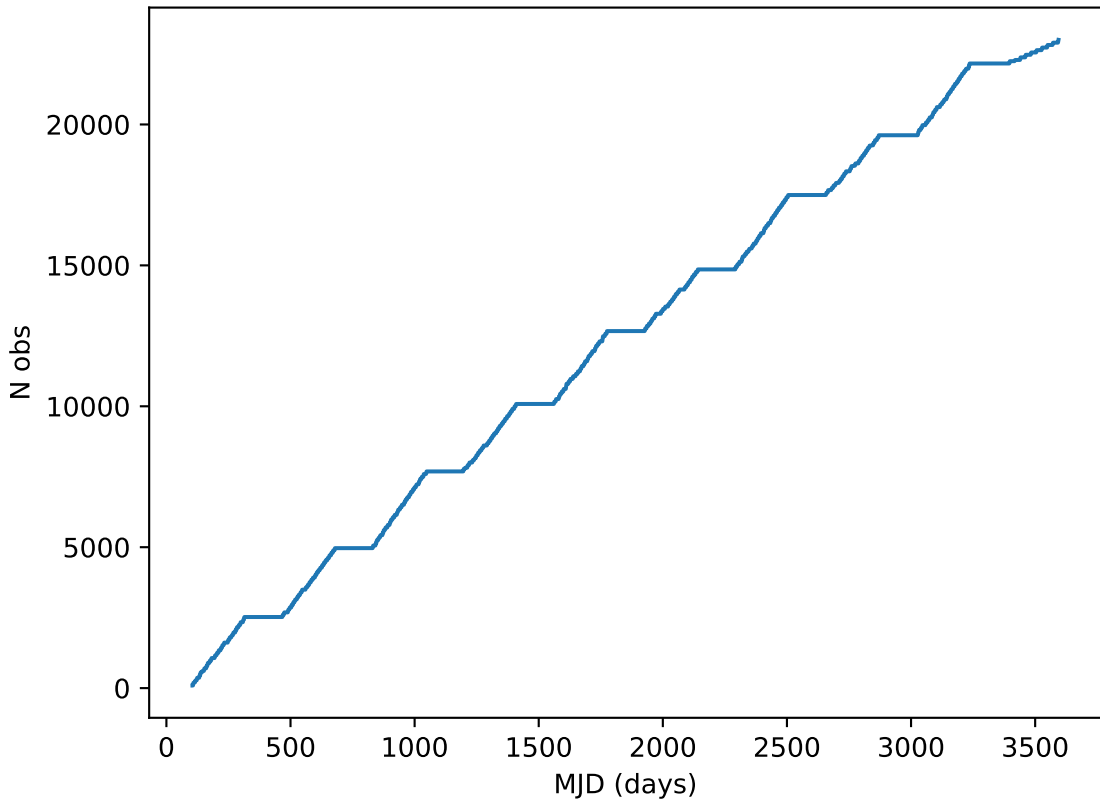
octo_v3.4_10yrs all bands: DD:EDFS Cumulative NVisits
