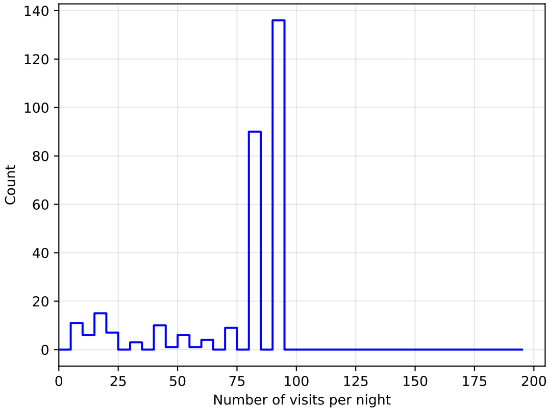
octo_v3.4_10yrs all bands: DD:ECDFS NVisitsPerNight
