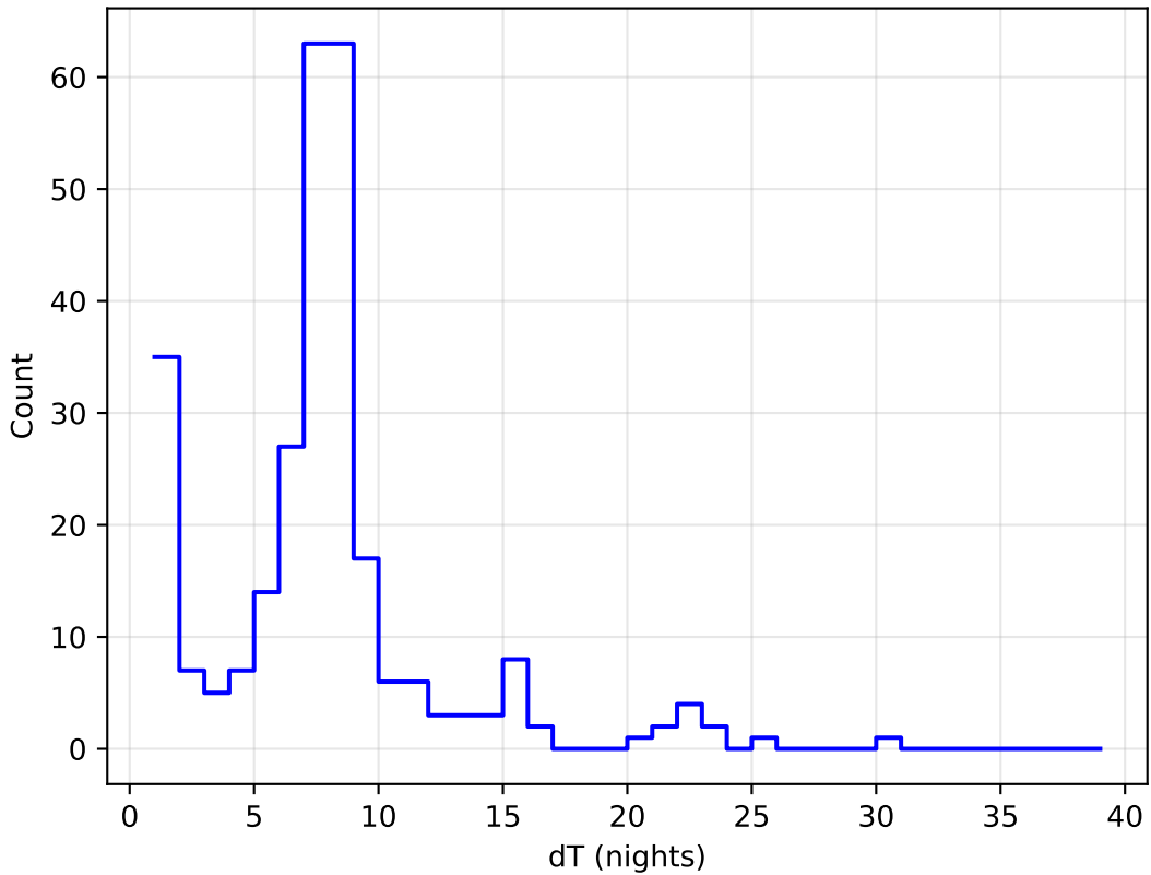
octo_v3.4_10yrs all bands: DD:ECDFS Delta Nights Histogram
