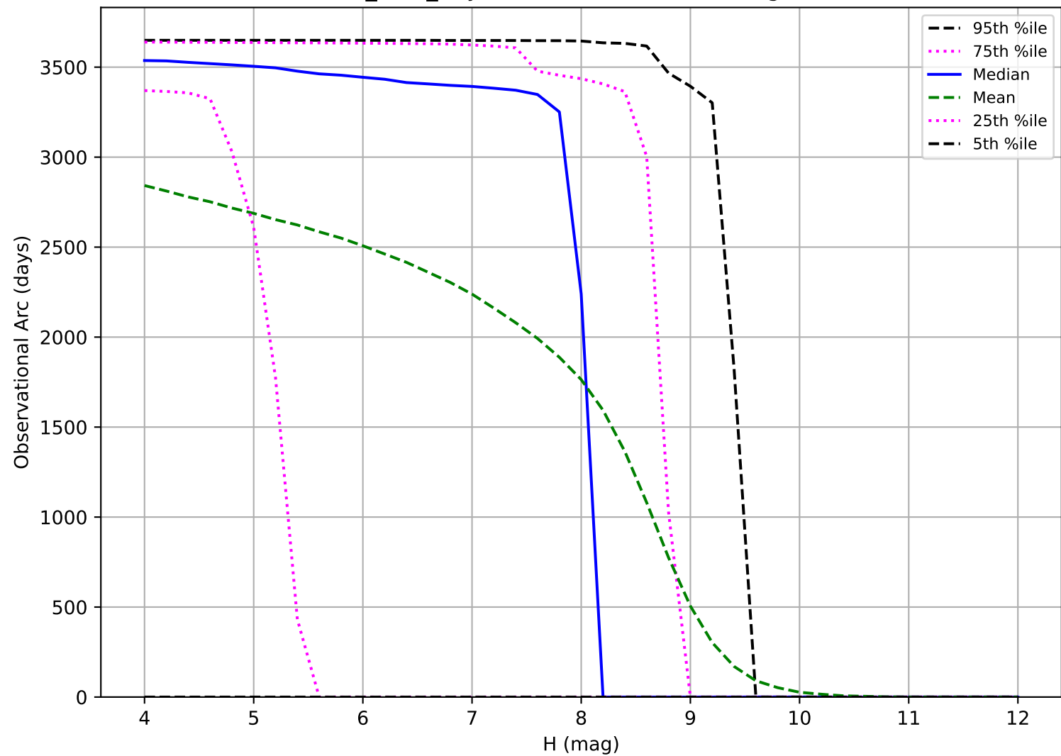
noroll_v3.4_10yrs: Observational Arc Length TNO
