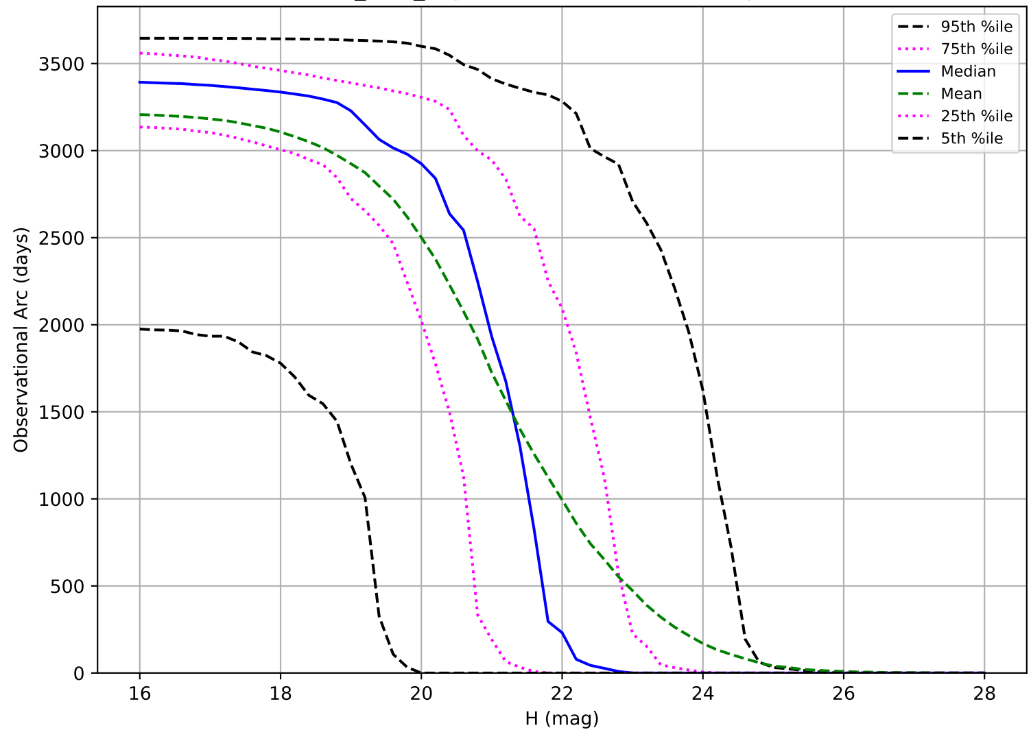
noroll_v3.4_10yrs: Observational Arc Length PHA
