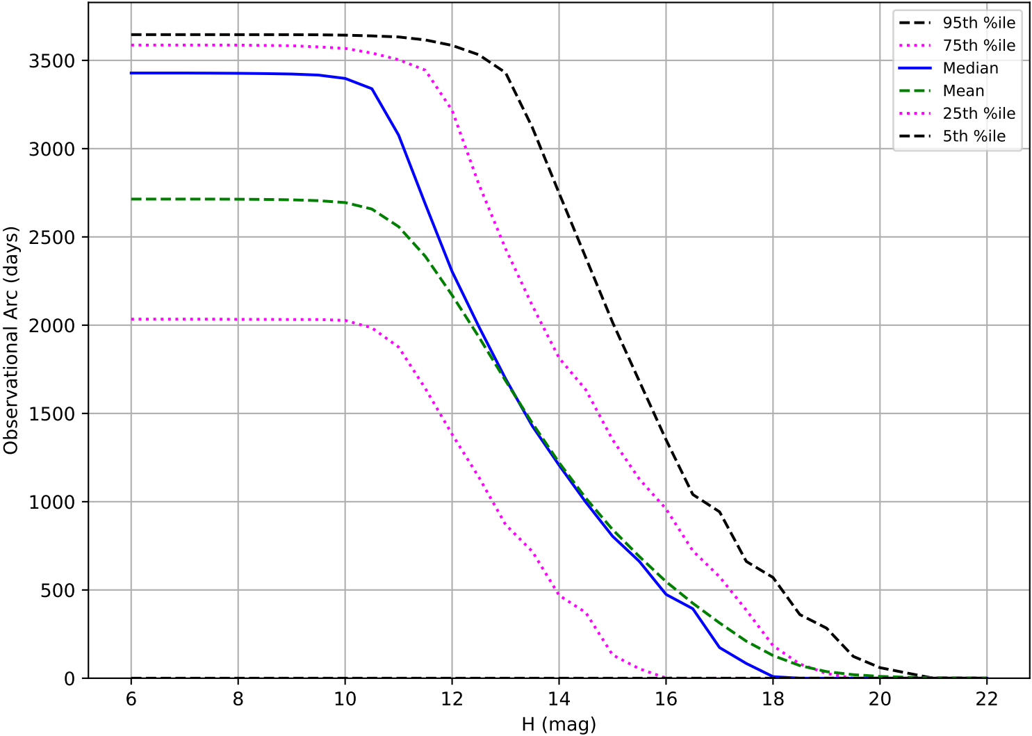
noroll_v3.4_10yrs: Observational Arc Length OCC_r5
