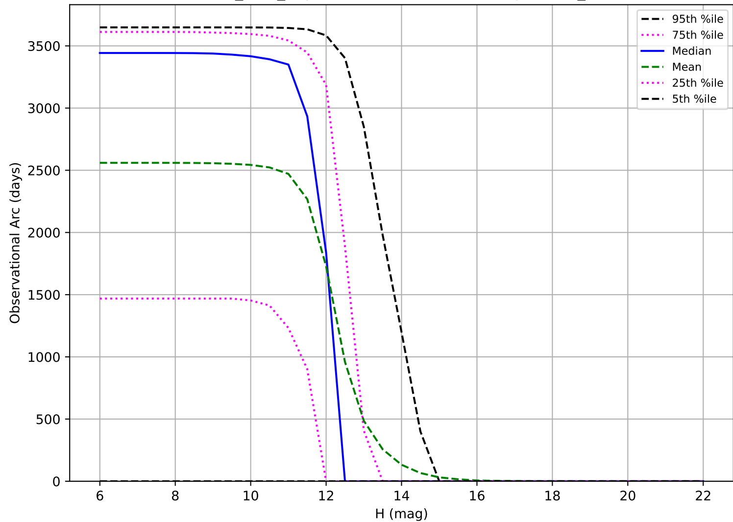
noroll_v3.4_10yrs: Observational Arc Length OCC_r20
