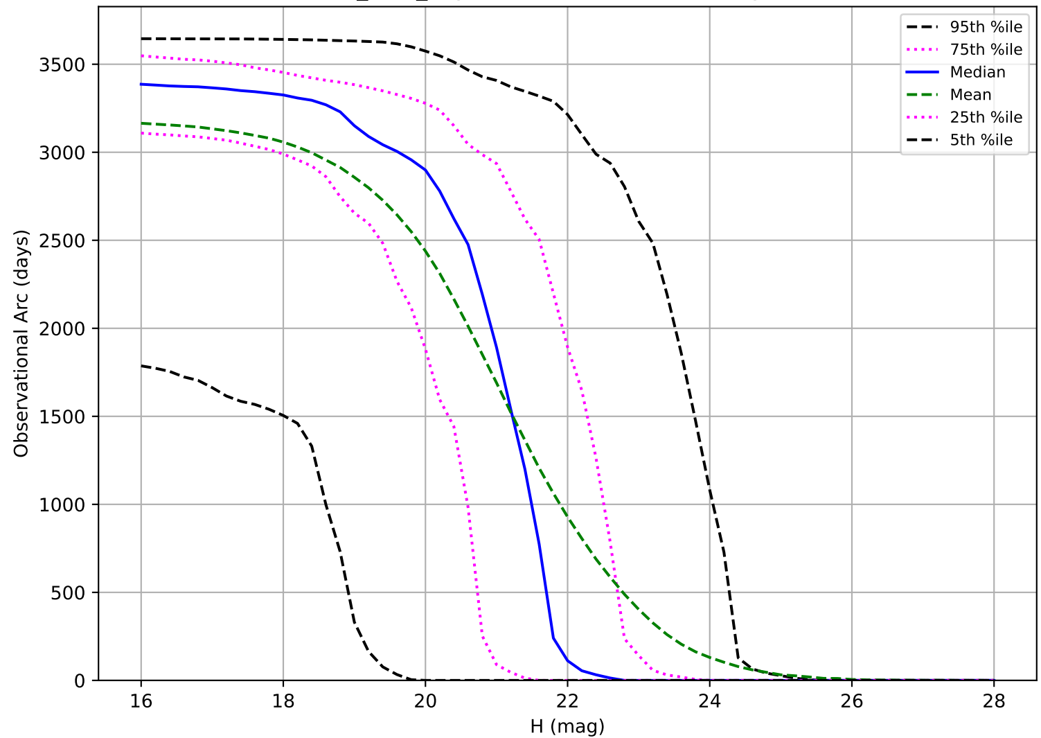
noroll_v3.4_10yrs: Observational Arc Length NEO
