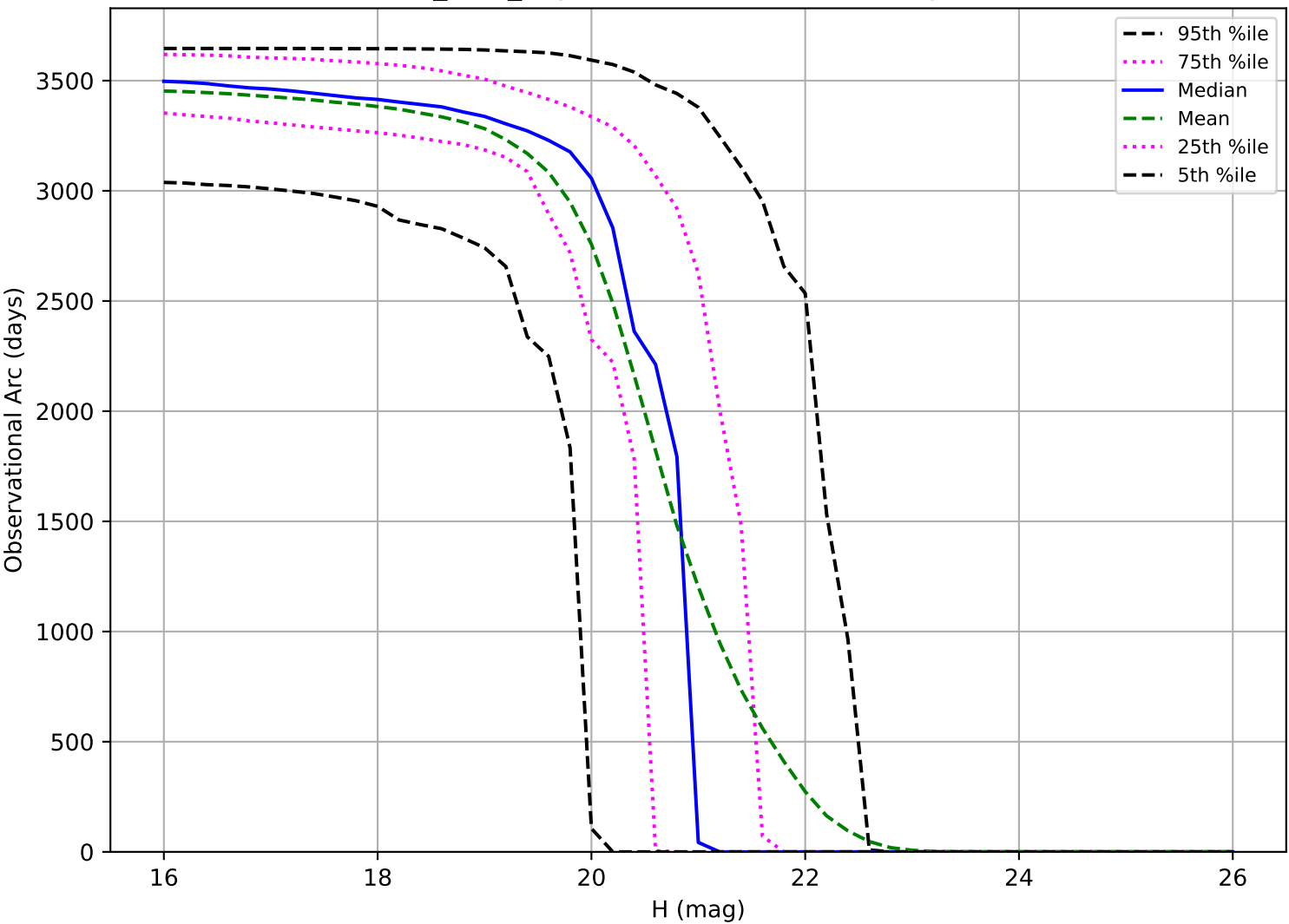
noroll_v3.4_10yrs: Observational Arc Length MBA
