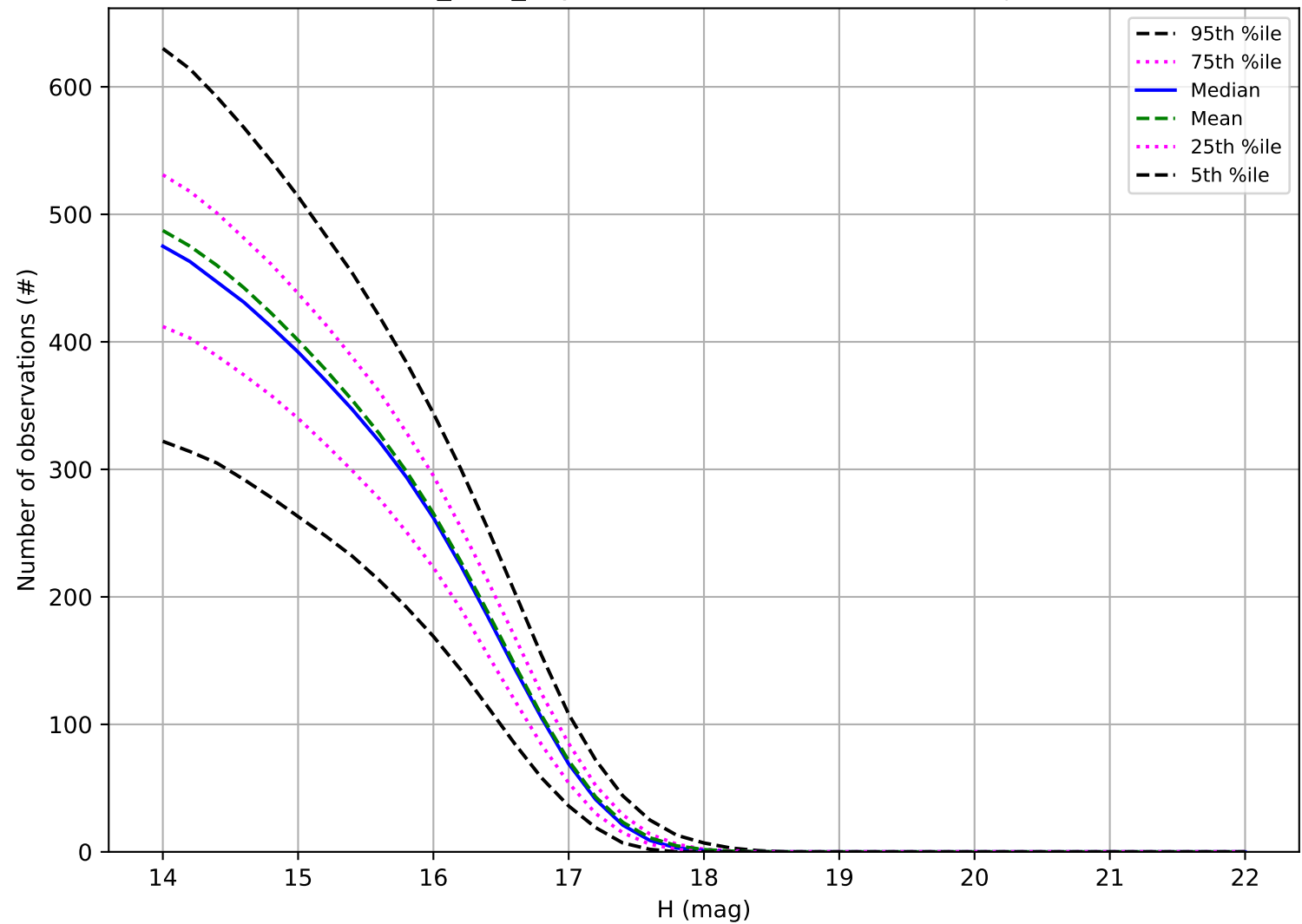
noroll_v3.4_10yrs: Number of observations Trojan
