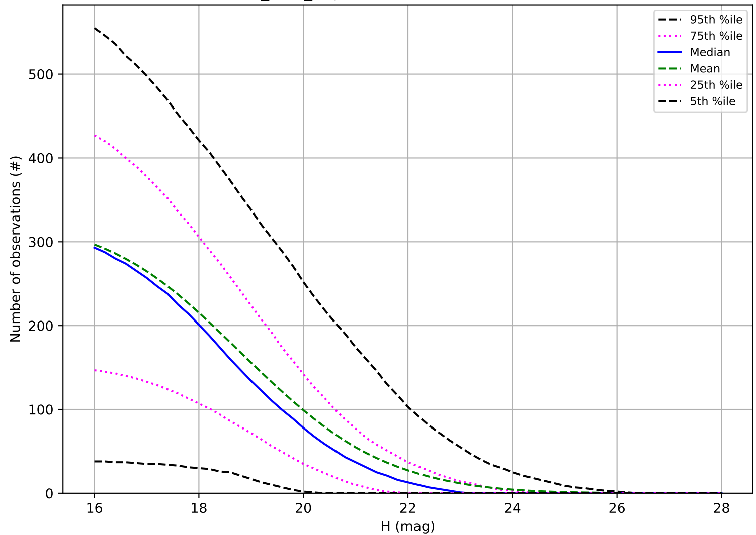
noroll_v3.4_10yrs: Number of observations PHA
