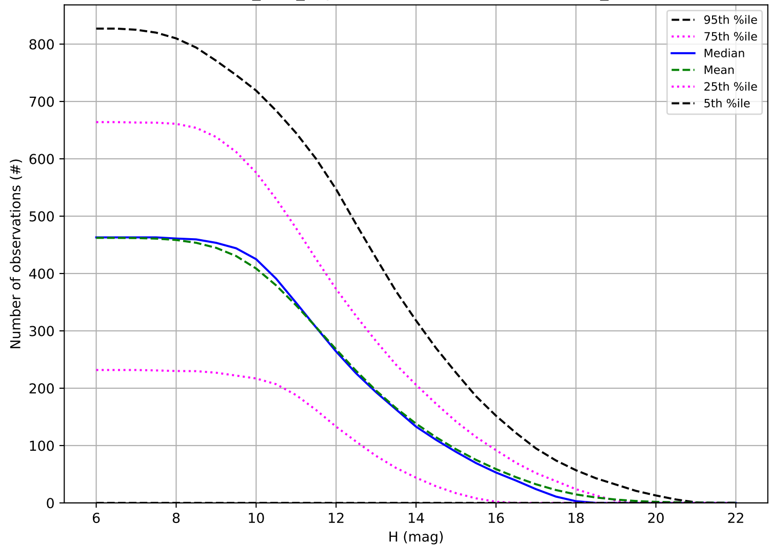
noroll_v3.4_10yrs: Number of observations OCC_r5
