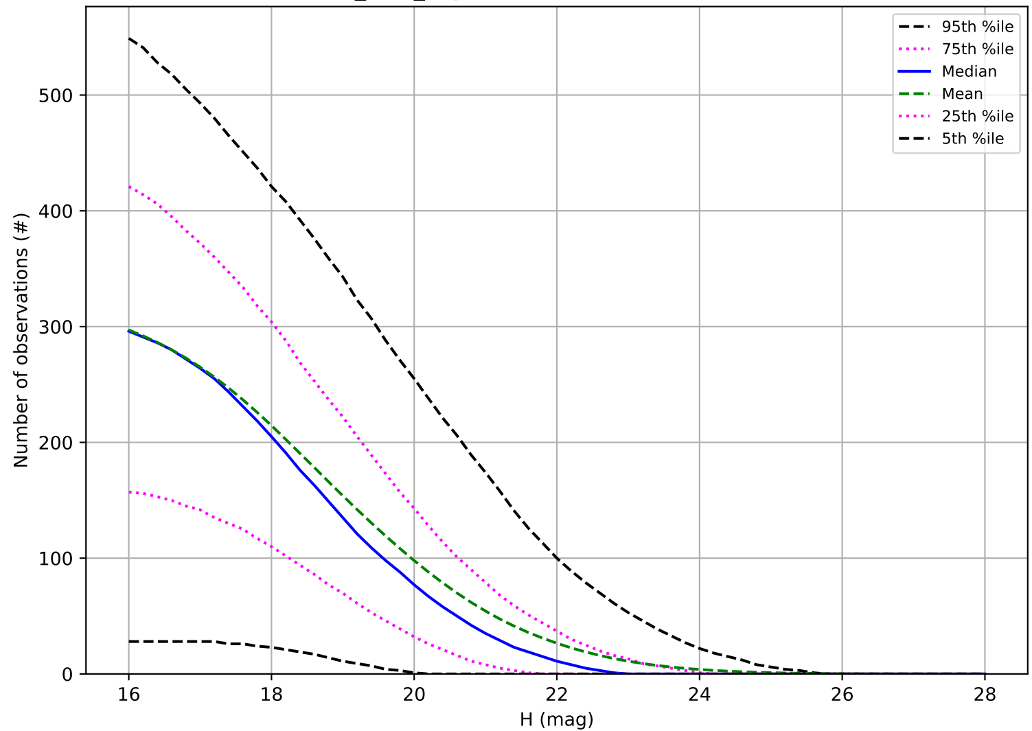
noroll_v3.4_10yrs: Number of observations NEO
