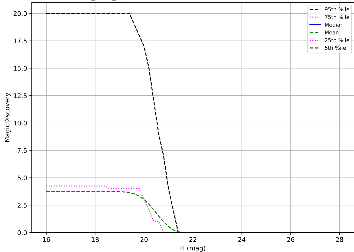
noroll_v3.4_10yrs: Vatira 6 detections in 60 nights detection loss
