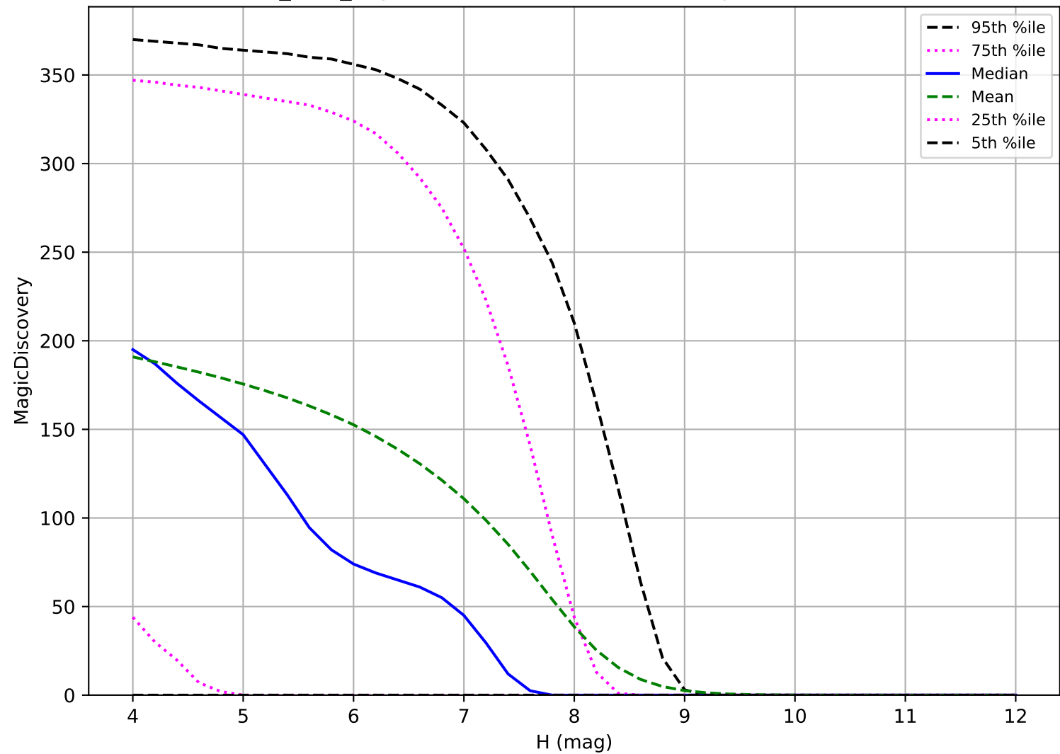
noroll_v3.4_10yrs: TNO 6 detections in 60 nights detection loss
