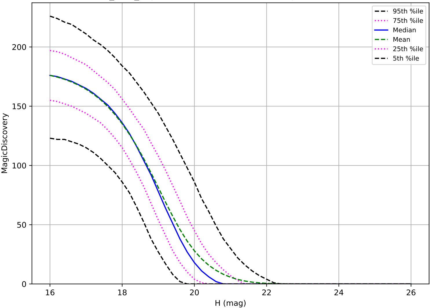
noroll_v3.4_10yrs: MBA 6 detections in 60 nights detection loss
