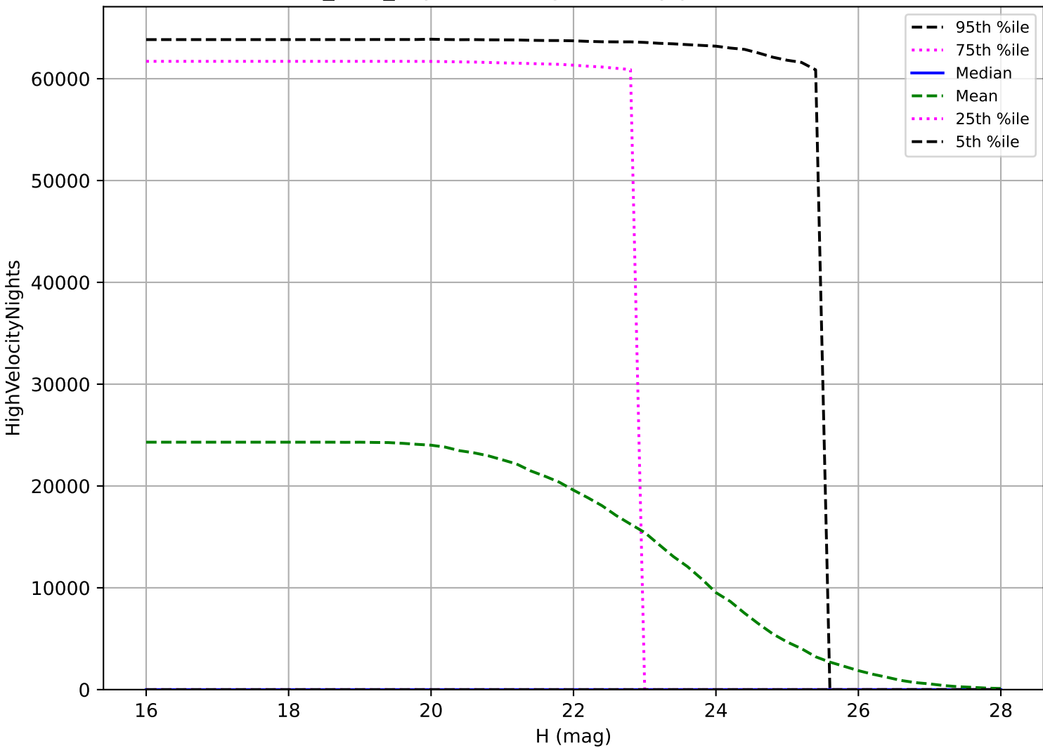
noroll_v3.4_10yrs: PHA High velocity pair detection loss
