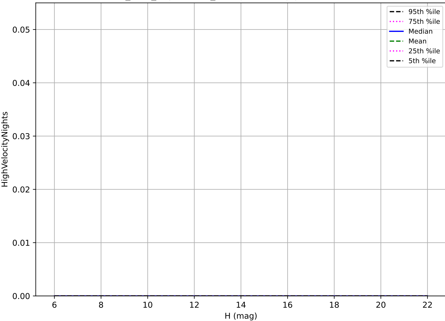
noroll_v3.4_10yrs: OCC_r5 High velocity pair detection loss
