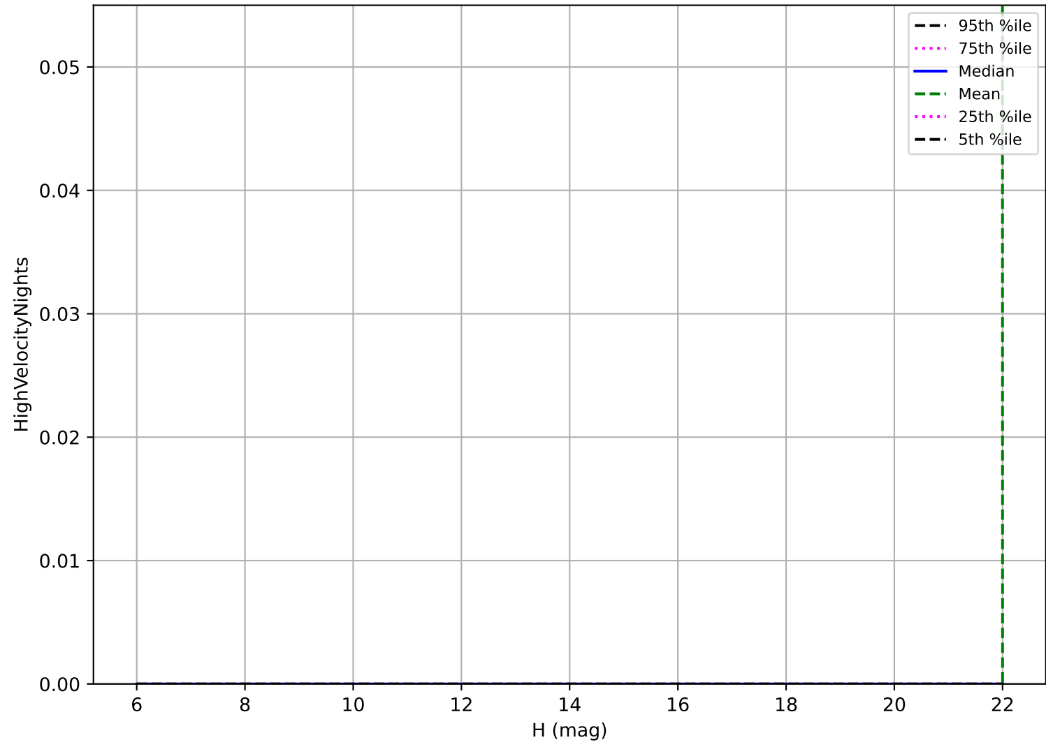
noroll_v3.4_10yrs: OCC_r20 High velocity pair detection loss
