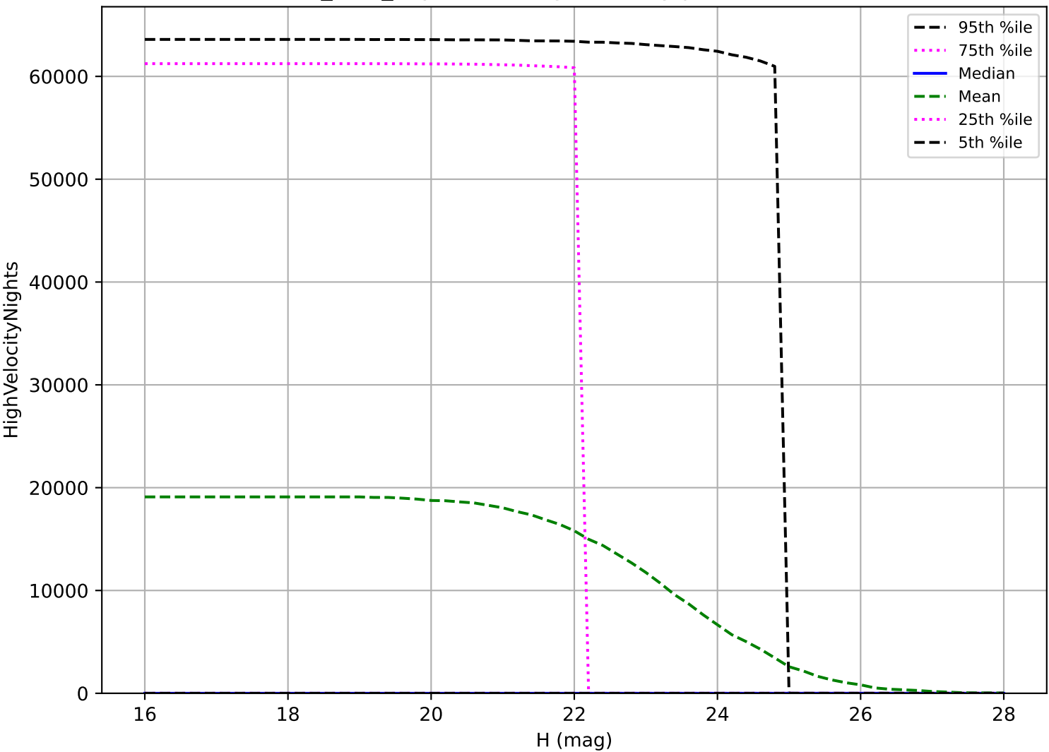
noroll_v3.4_10yrs: NEO High velocity pair detection loss
