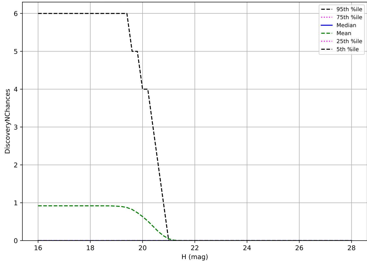
noroll_v3.4_10yrs: Vatira 3 pairs in 15 nights detection loss
