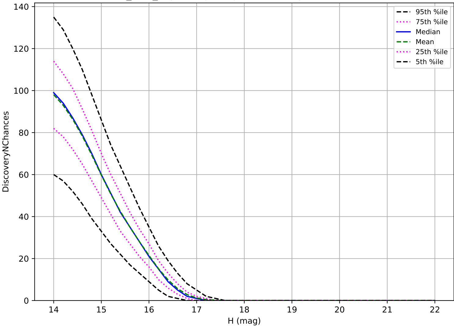
noroll_v3.4_10yrs: Trojan 3 pairs in 15 nights detection loss
