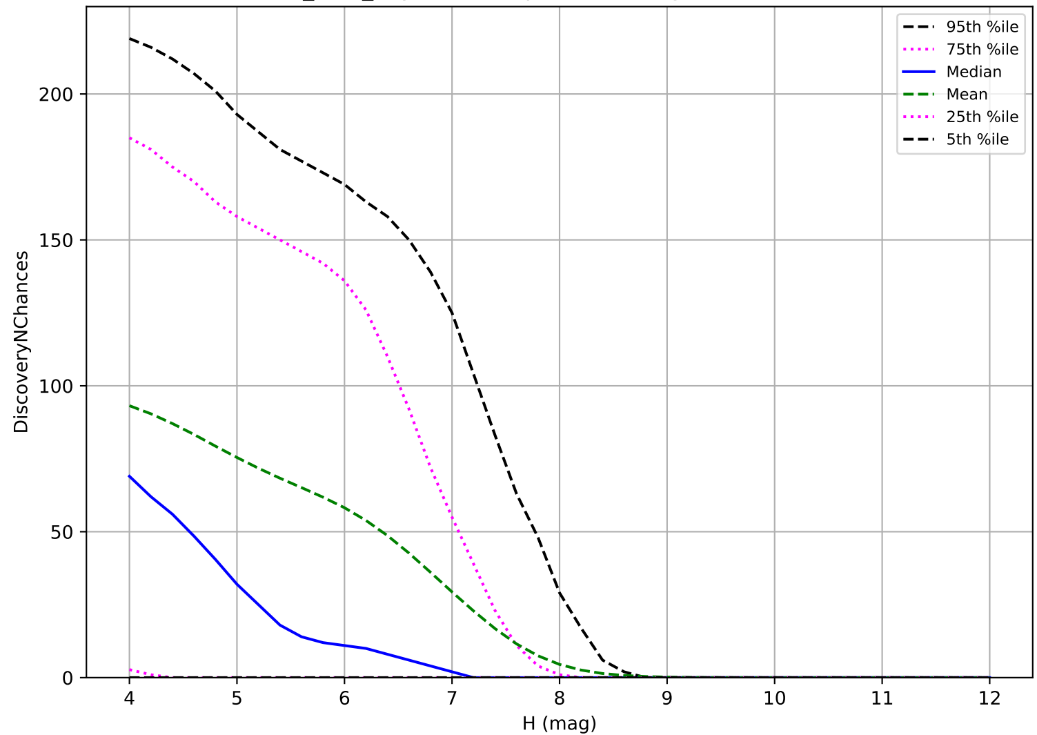
noroll_v3.4_10yrs: TNO 3 pairs in 15 nights detection loss
