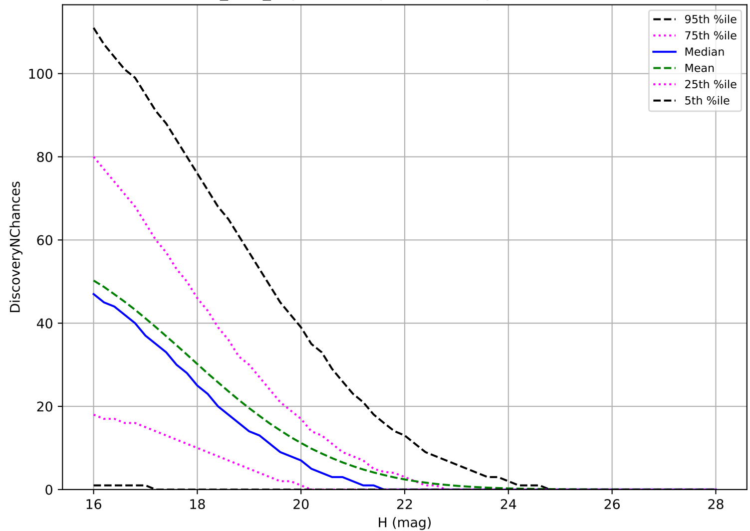
noroll_v3.4_10yrs: PHA 3 pairs in 15 nights detection loss
