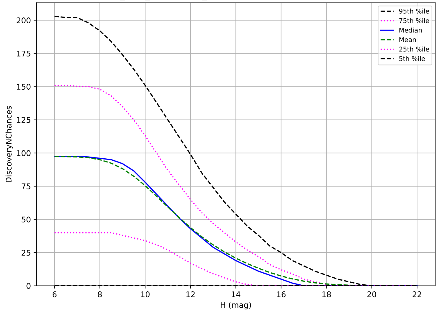
noroll_v3.4_10yrs: OCC_r5 3 pairs in 15 nights detection loss
