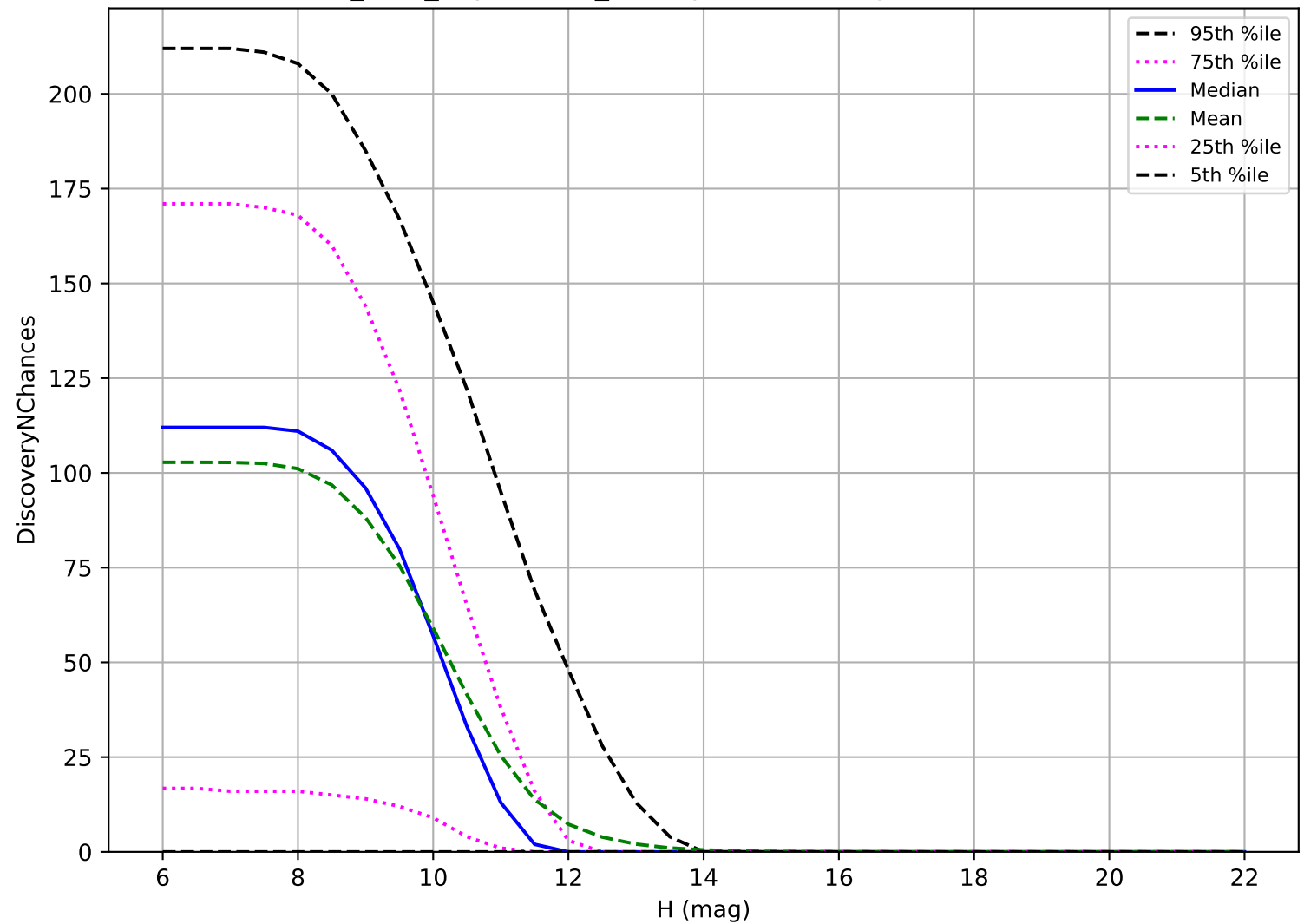
noroll_v3.4_10yrs: OCC_r20 3 pairs in 15 nights detection loss
