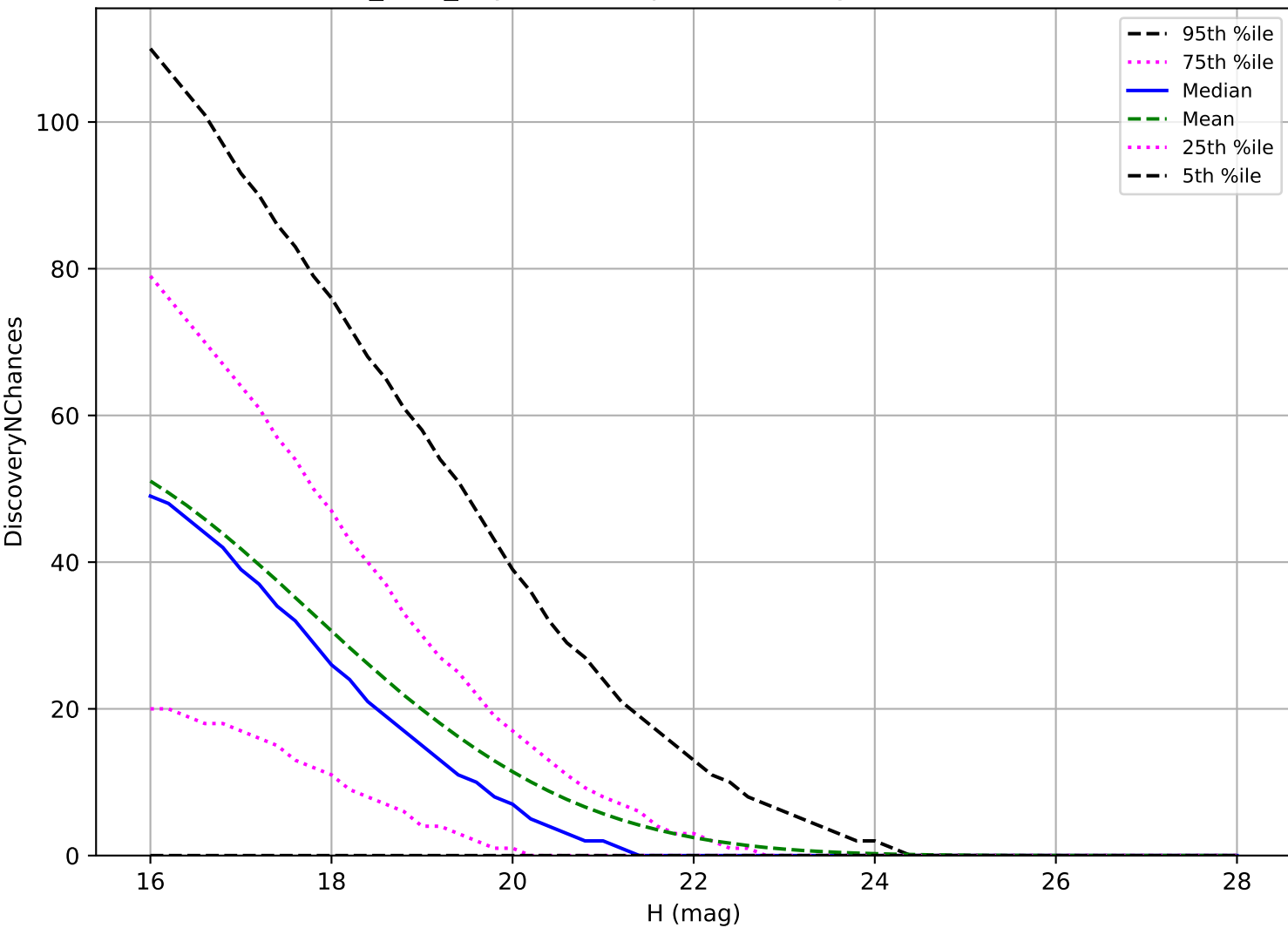
noroll_v3.4_10yrs: NEO 3 pairs in 15 nights detection loss
