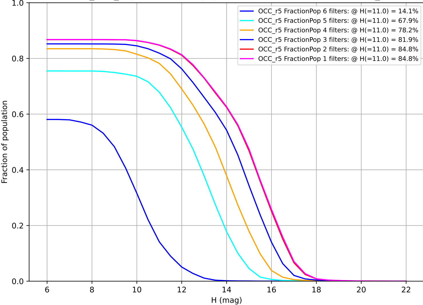
noroll_v3.4_10yrs: Fraction of population with colors in X filters OCC_r5
