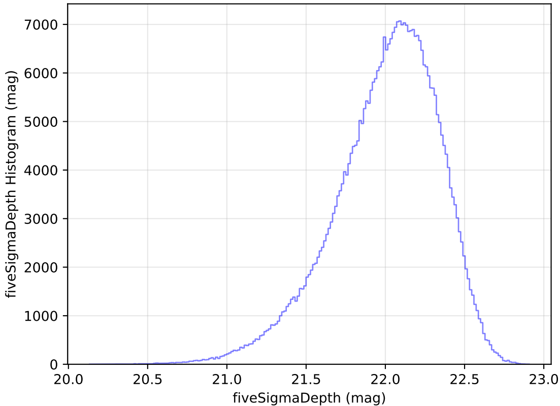
noroll_v3.4_10yrs y: fiveSigmaDepth Histogram
