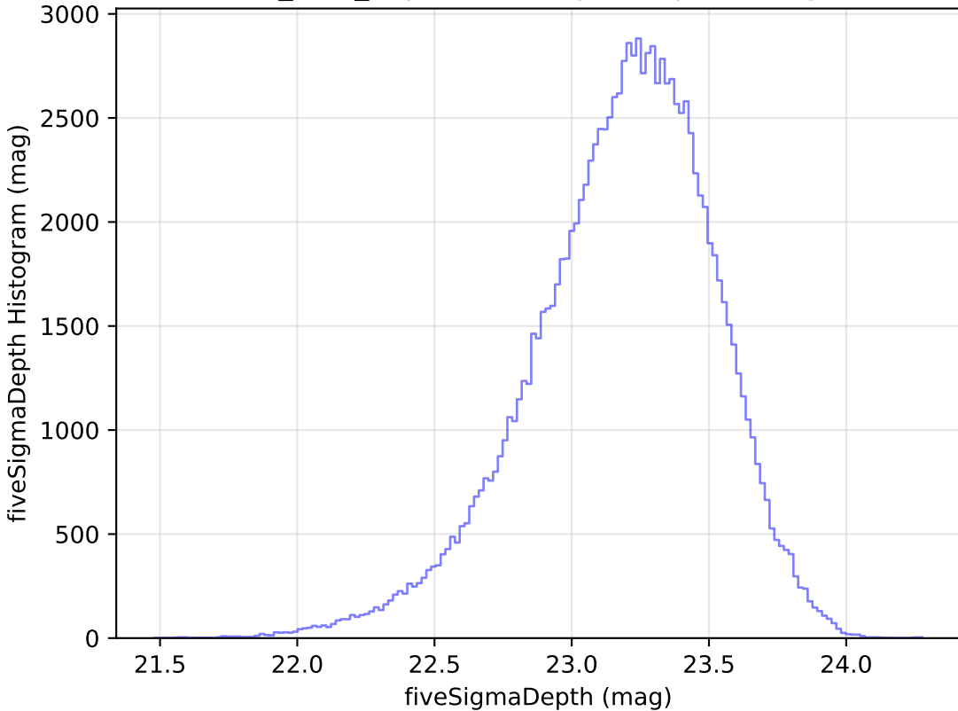
noroll_v3.4_10yrs u: fiveSigmaDepth Histogram
