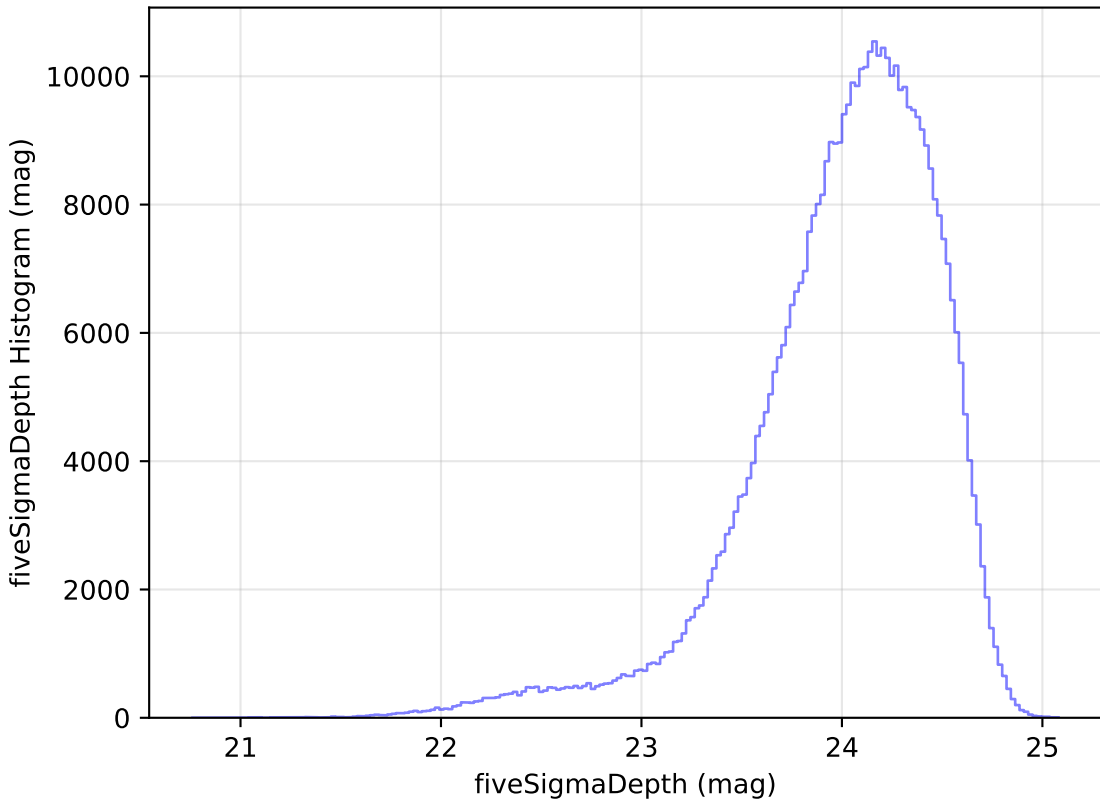
noroll_v3.4_10yrs r: fiveSigmaDepth Histogram
