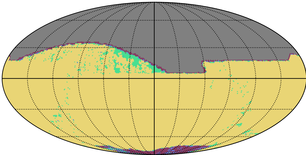
noroll_v3.4_10yrs z band: YearCoverage night
