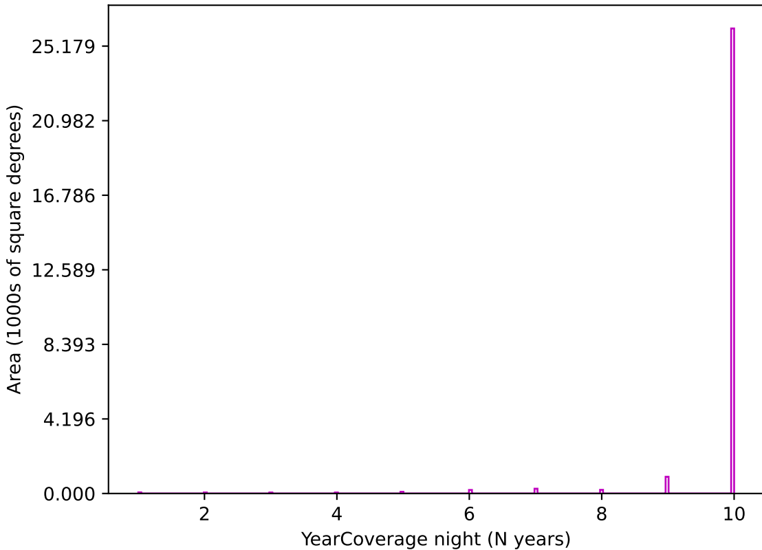
noroll_v3.4_10yrs z band: YearCoverage night
