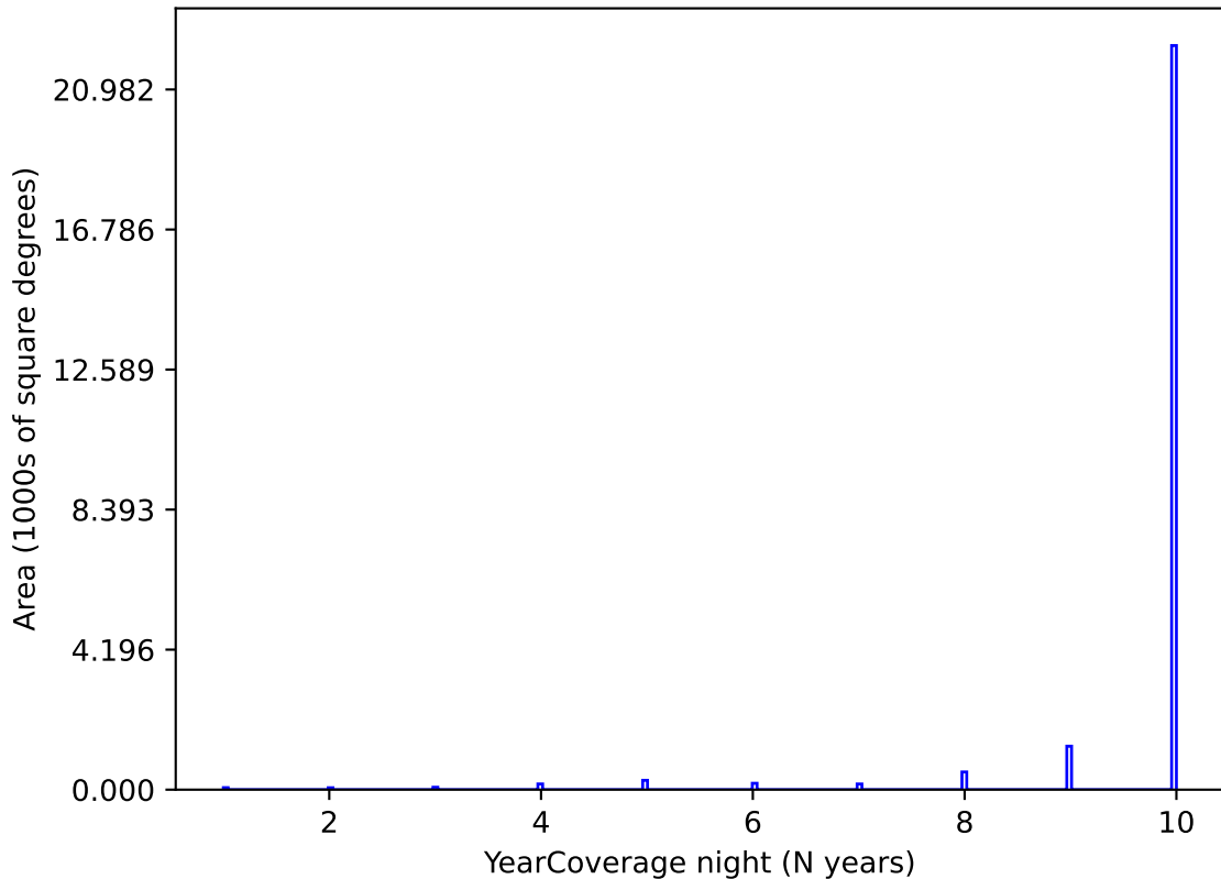
noroll_v3.4_10yrs y band: YearCoverage night
