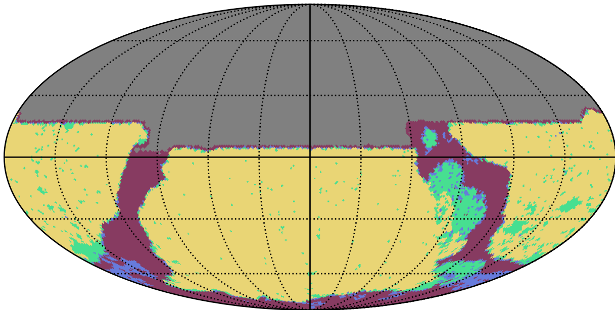
noroll_v3.4_10yrs u band: YearCoverage night
