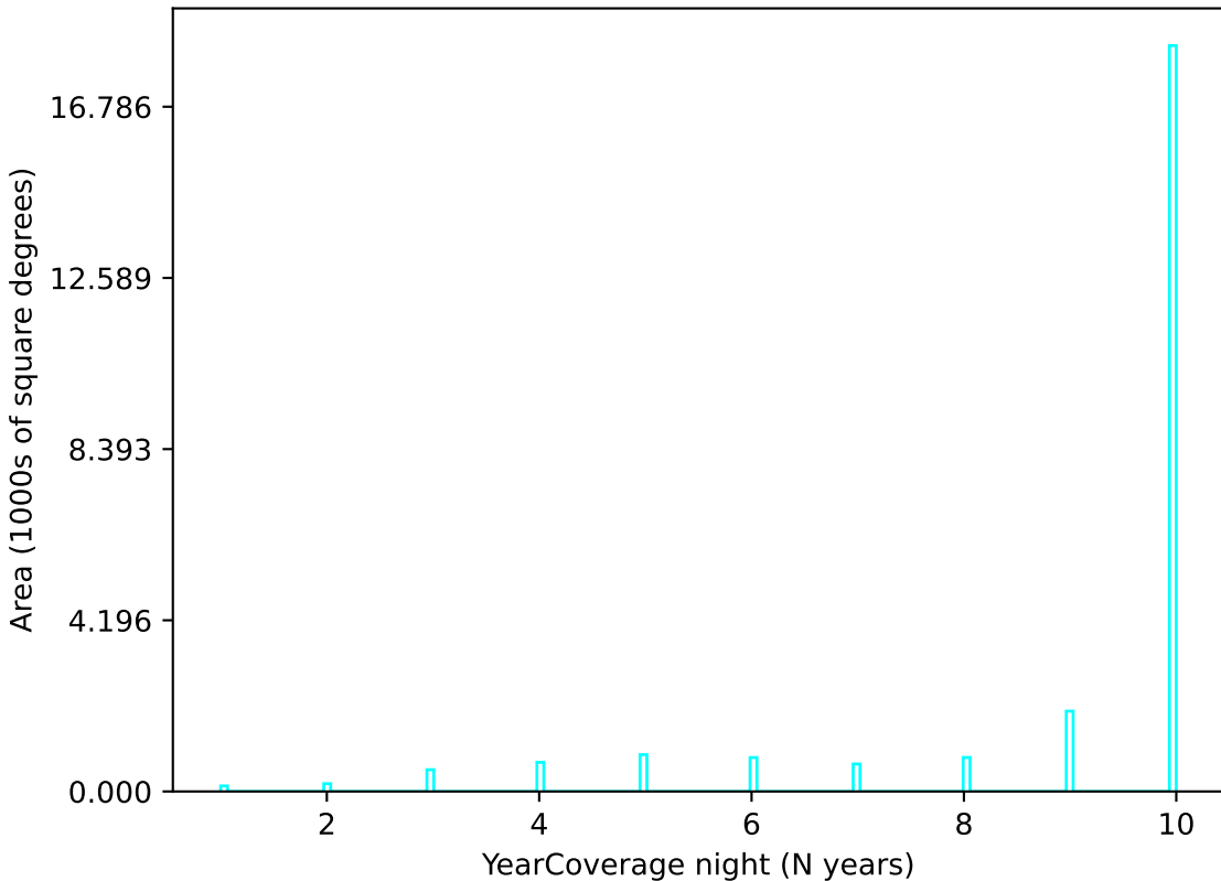
noroll_v3.4_10yrs u band: YearCoverage night
