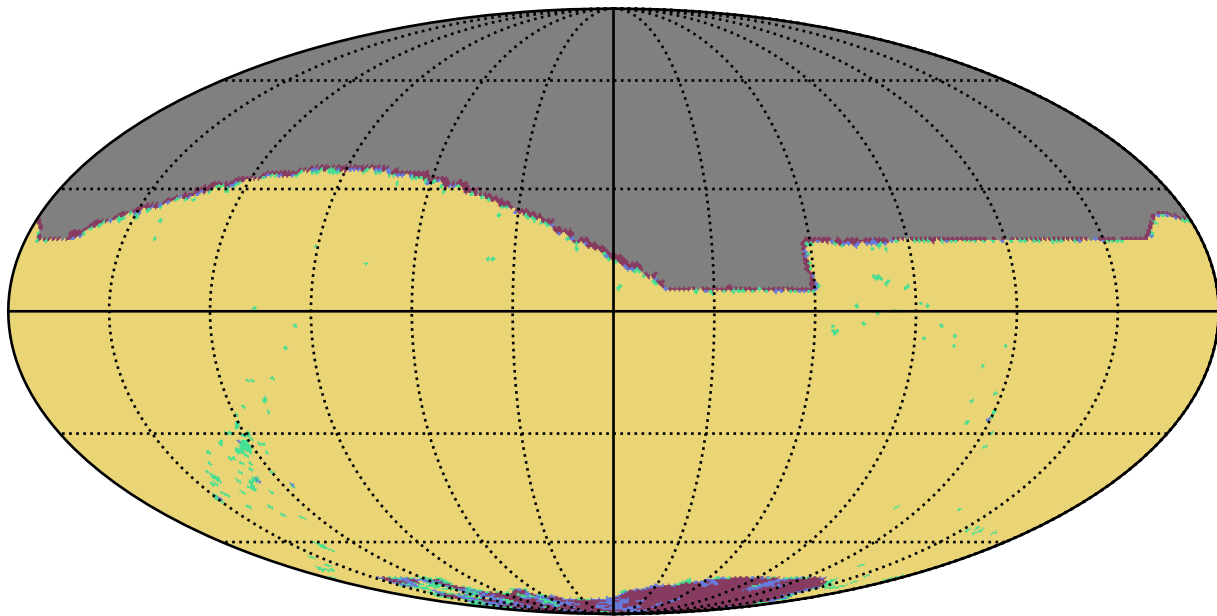
noroll_v3.4_10yrs r band: YearCoverage night
