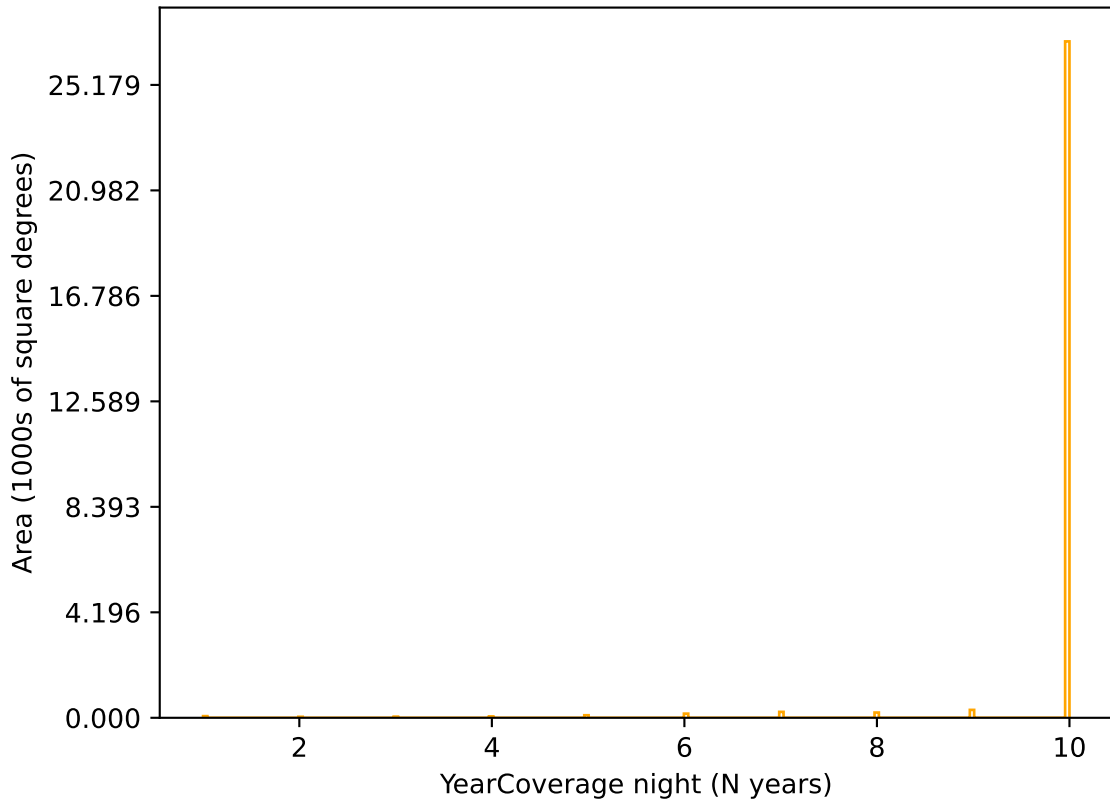
noroll_v3.4_10yrs r band: YearCoverage night
