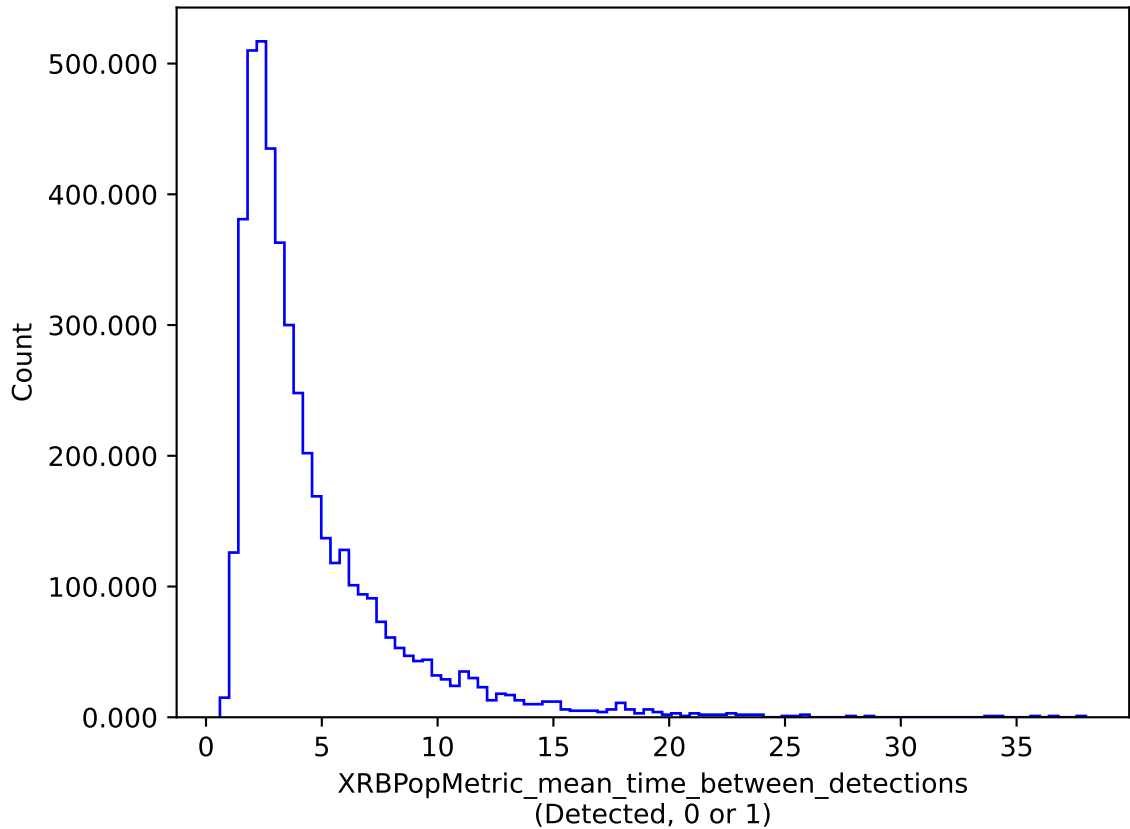
noroll_v3.4_10yrs : XRBPoMetric_mean_time_between_detections
