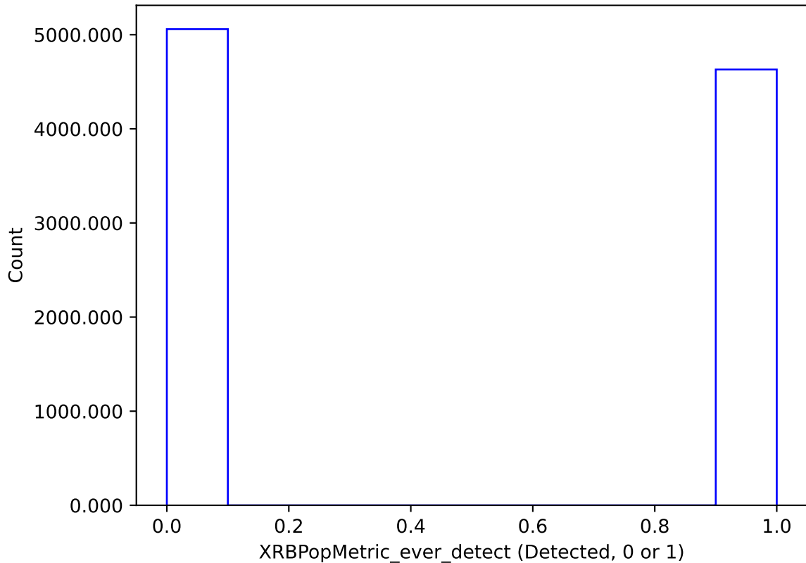
noroll_v3.4_10yrs : XRBPoMetric_ever_detect
