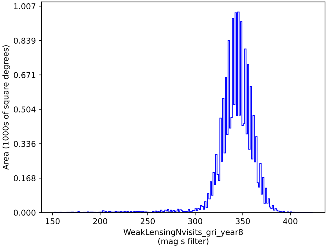
noroll_v3.4_10yrs gri band non-DD: WeakLensingNvisits_gri_year8
