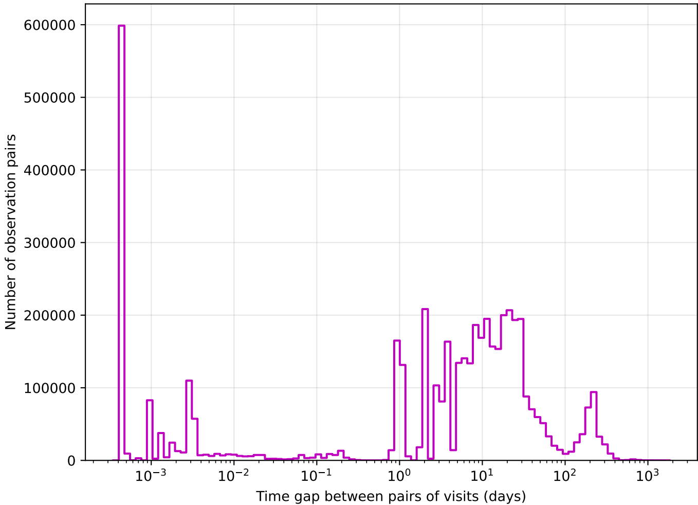
noroll_v3.4_10yrs z band: Tgaps observationStartMJD
