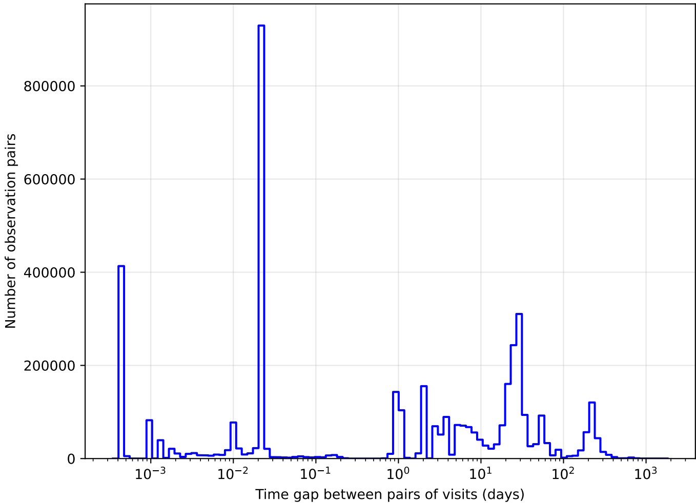
noroll_v3.4_10yrs y band: Tgaps observationStartMJD
