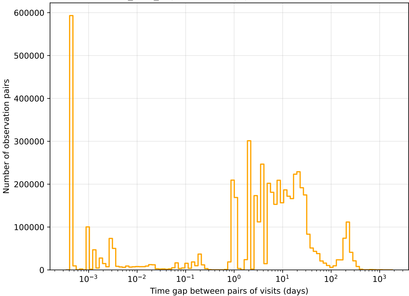
noroll_v3.4_10yrs r band: Tgaps observationStartMJD
