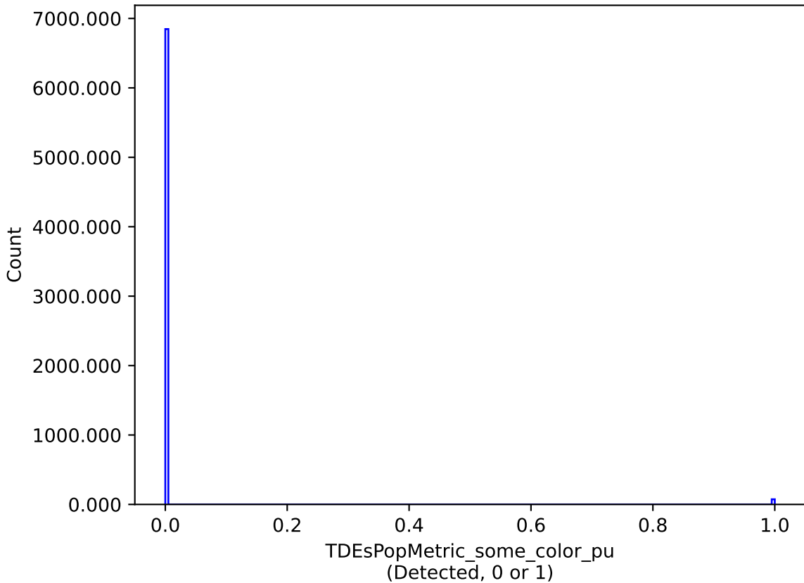
noroll_v3.4_10yrs : TDEsPopMetric_some_color_pu
