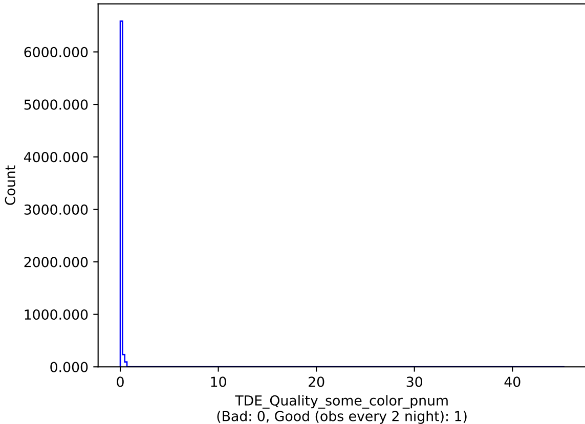
noroll_v3.4_10yrs : TDE_Quality_some_color_pnum
