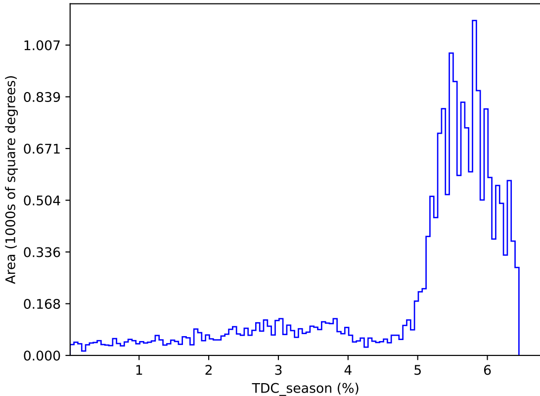
noroll_v3.4_10yrs : TDC_season
